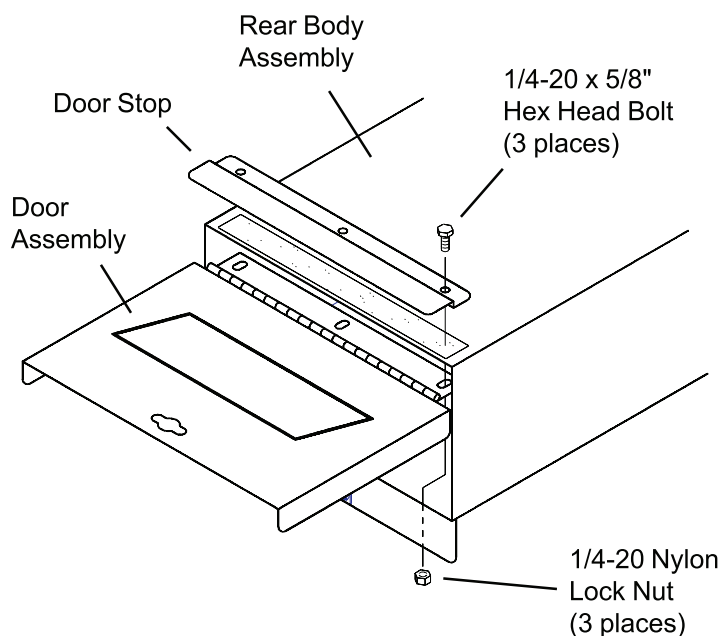
Figure 3. Door Stop and Door to Body Assembly
